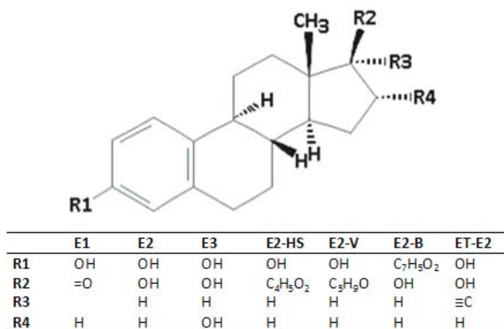
Fig. 1. Chemical structure of natural and synthetic estrogens.
